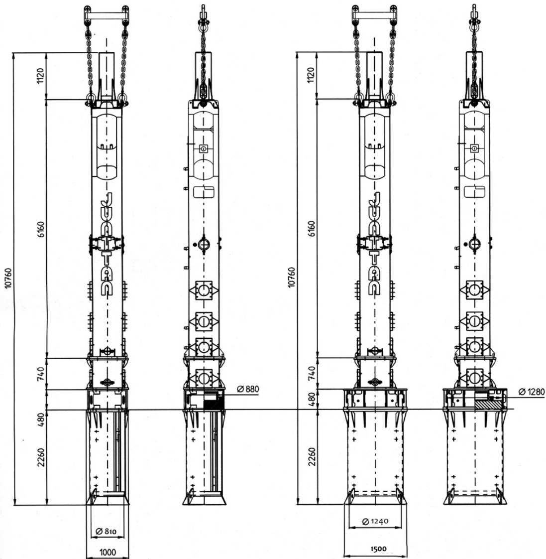
Pile Sleeve Ø 810
