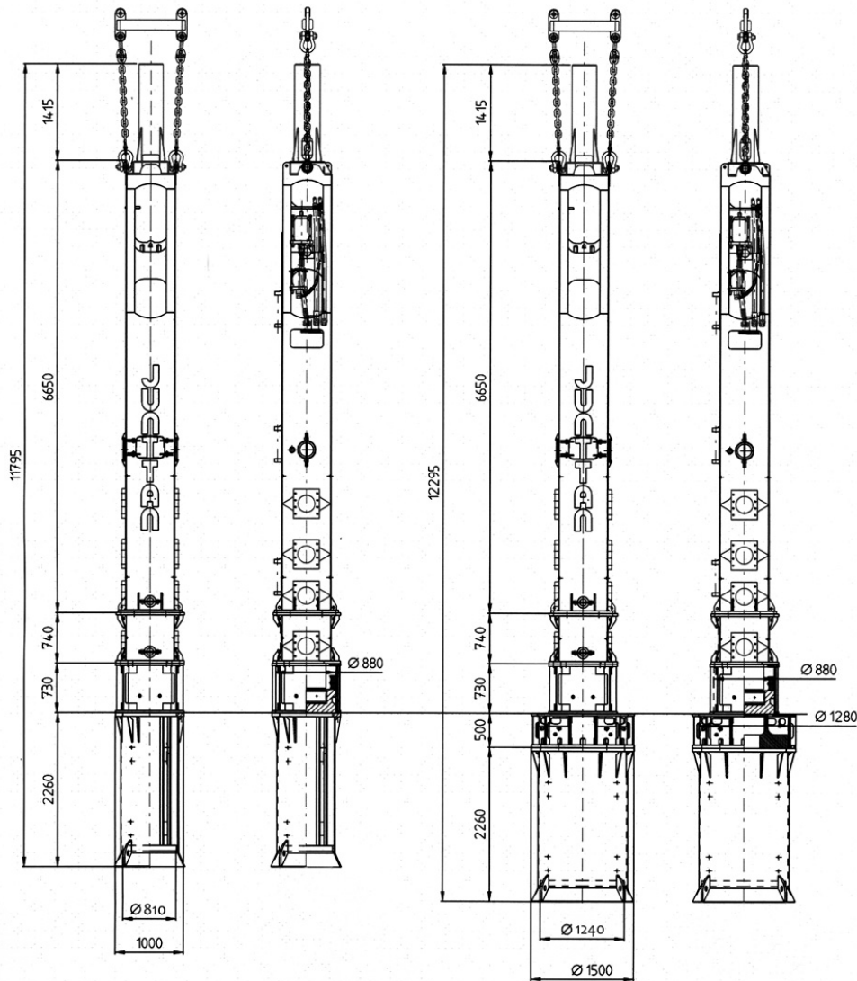
Pile Sleeve Ø 810
